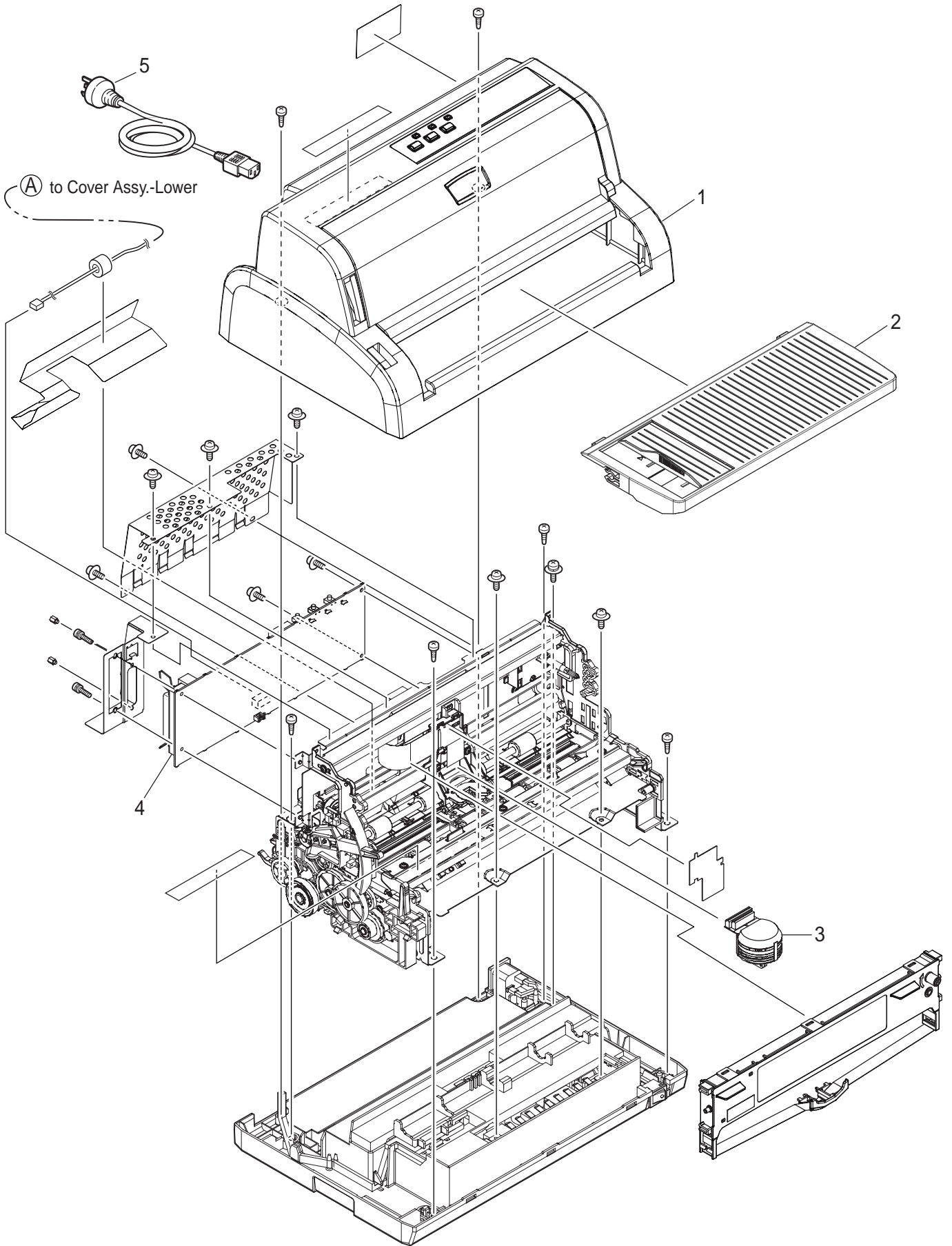
Printer SIDM
