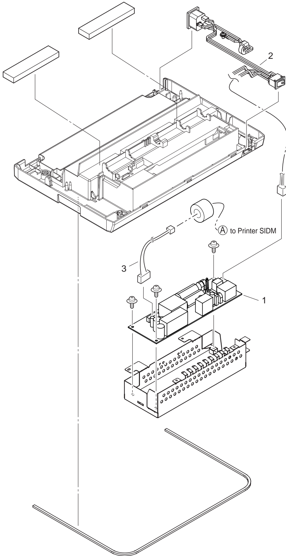
Cover Assy. - Lower
